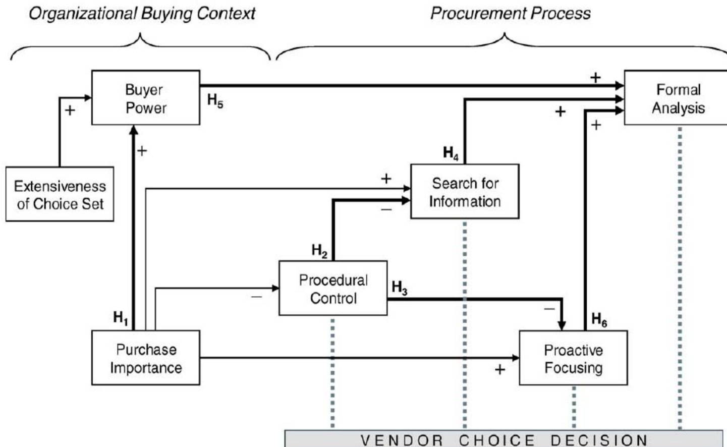
Fig. 1. Schematic overview of conceptual model. Bold lines highlight 6 focal hypothesized relationships between constructs; other (lighter) lines indicate relationships included for control.
